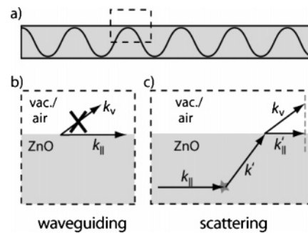
Figure 5. Polariton guiding in a ZnO nanowire. (a) Schematic of a standing-wave polariton in a wire. (b) Magnification of the ZnO/air interface; modes with k_{\parallel} larger than the wavevector k_v in free space (at the same energy) cannot escape through the sides of the wire and are hence guided. (c) Exciton polariton modes that are scattered may escape through the sides of the wire ( k' is the wavevector of the scattered mode, with a parallel projection k'_{\parallel} ).
